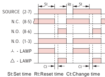
N Type
