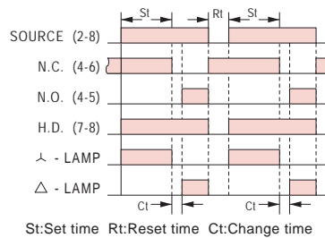
T Type
